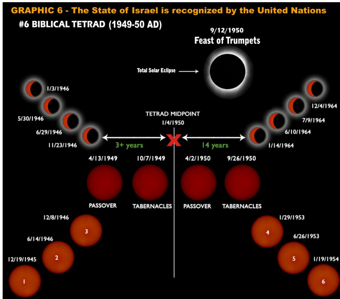
Graphic 6: Biblical Blood Moon Tetrad during 1949-1950. There were 3 total lunar eclipses before and another 3 thereafter. There were also 4 partial solar eclipses before and another 4 thereafter. There was also a total solar eclipse at the Feast of Trumpets.
