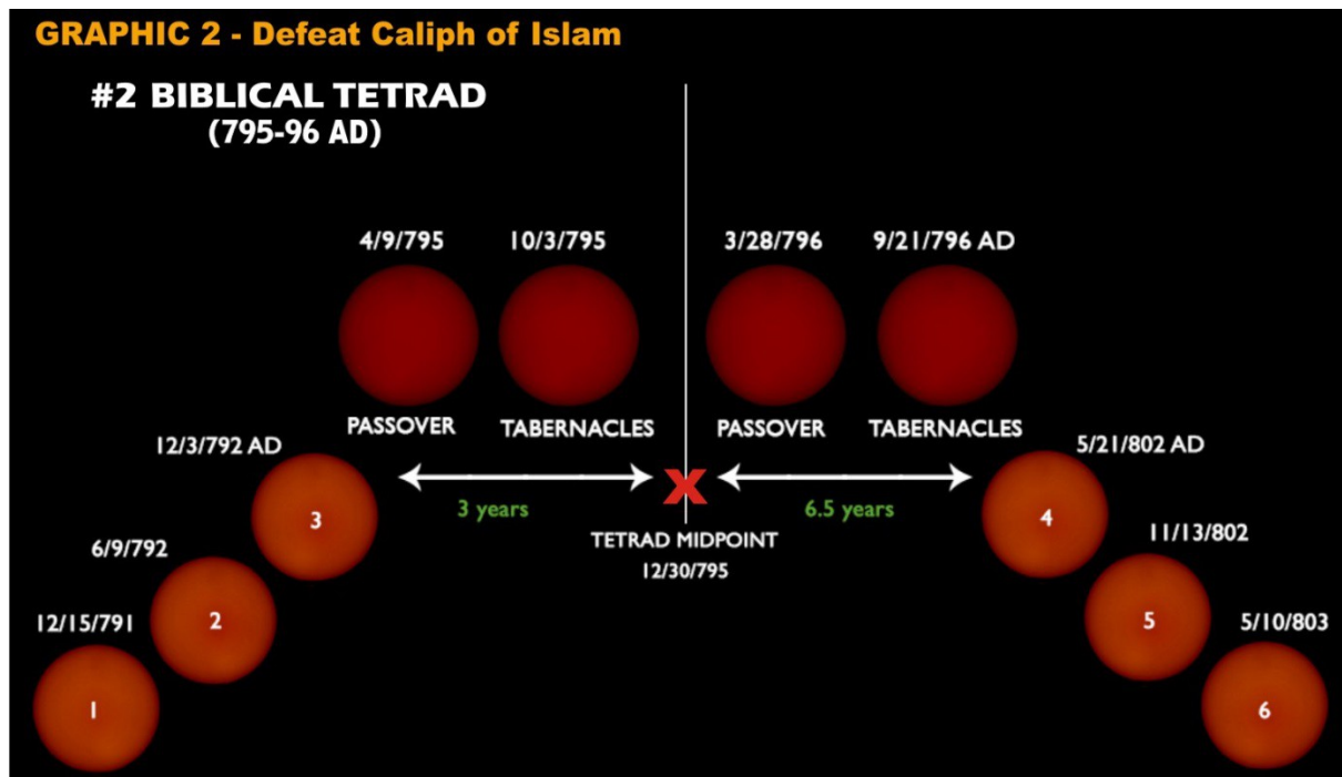
Graphic 2: Biblical Blood Moon Tetrad during 795-796 AD. There were 3 total lunar eclipses before and 3 others thereafter.
