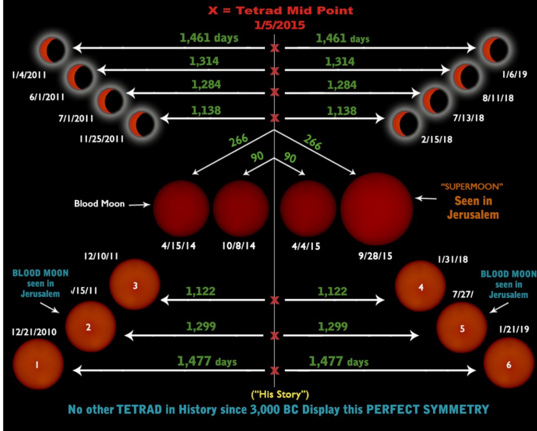
Graphic 8 A: Biblical Blood Moon Tetrad during 2014-2015. There were 3 total lunar eclipses before and there will be another 3 thereafter. There were also 4 partial solar eclipses before and there will be another 4 thereafter.
