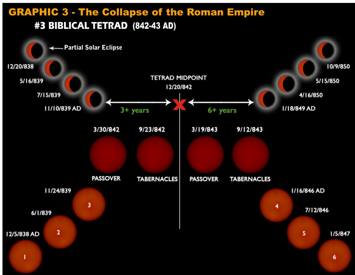
Graphic 3: Biblical Blood Moon Tetrad during 842-843 AD. There were 3 total lunar eclipses before and another 3 thereafter. There were also 4 partial solar eclipses before and another 4 thereafter .
